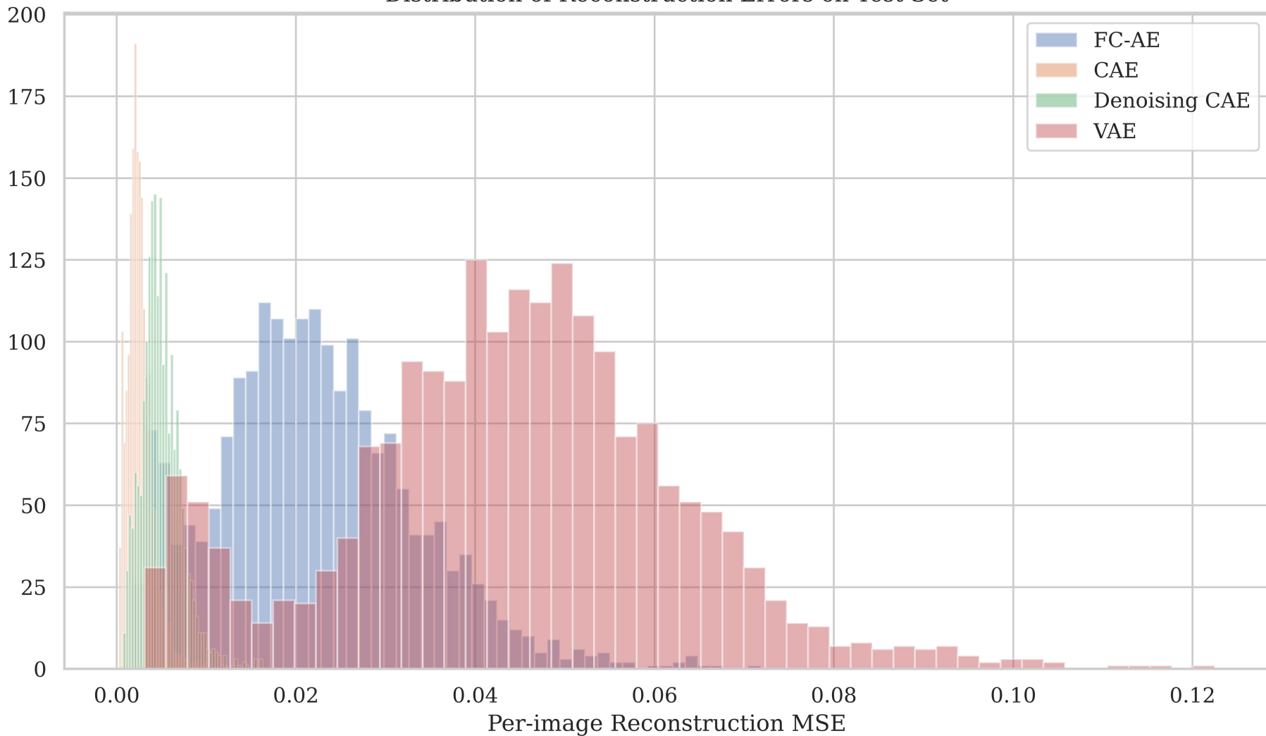
Distribution of Reconstruction Errors on Test Set
